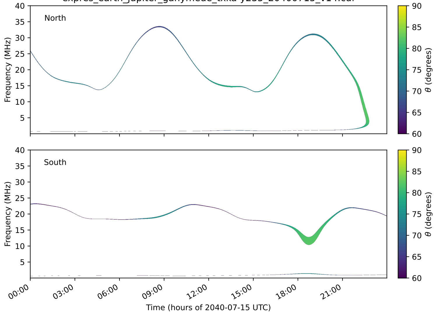
expres_earth_jupiter_ganymede_txka-y235_20400715_v14.cdf
