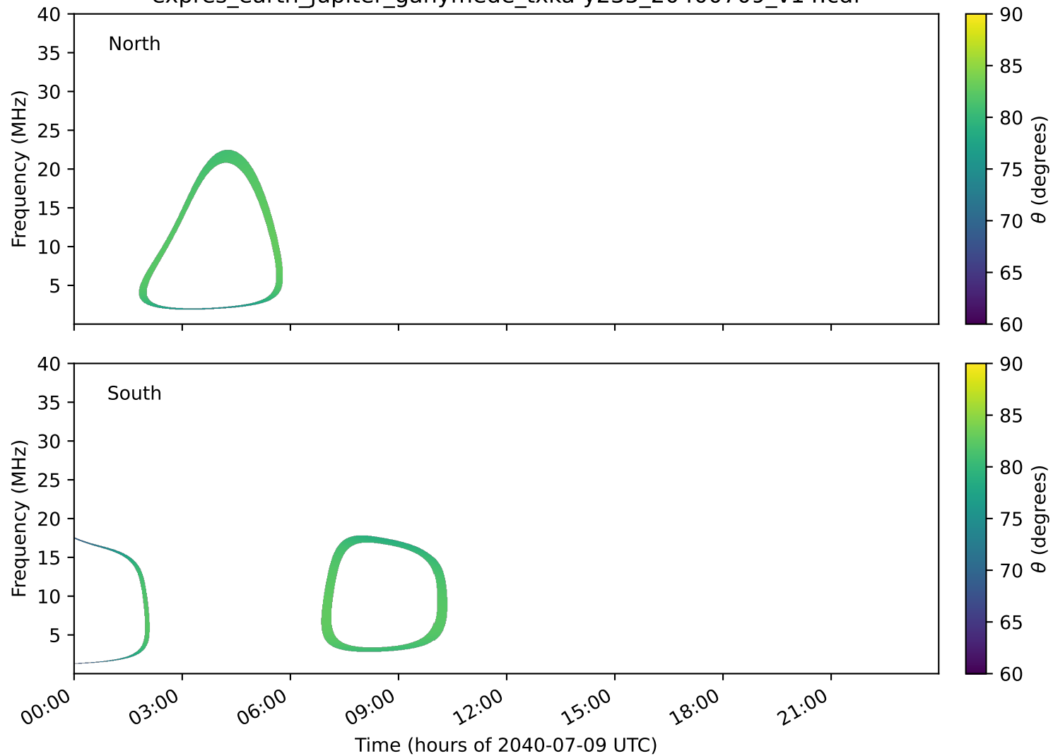
expres_earth_jupiter_ganymede_txka-y235_20400709_v14.cdf
