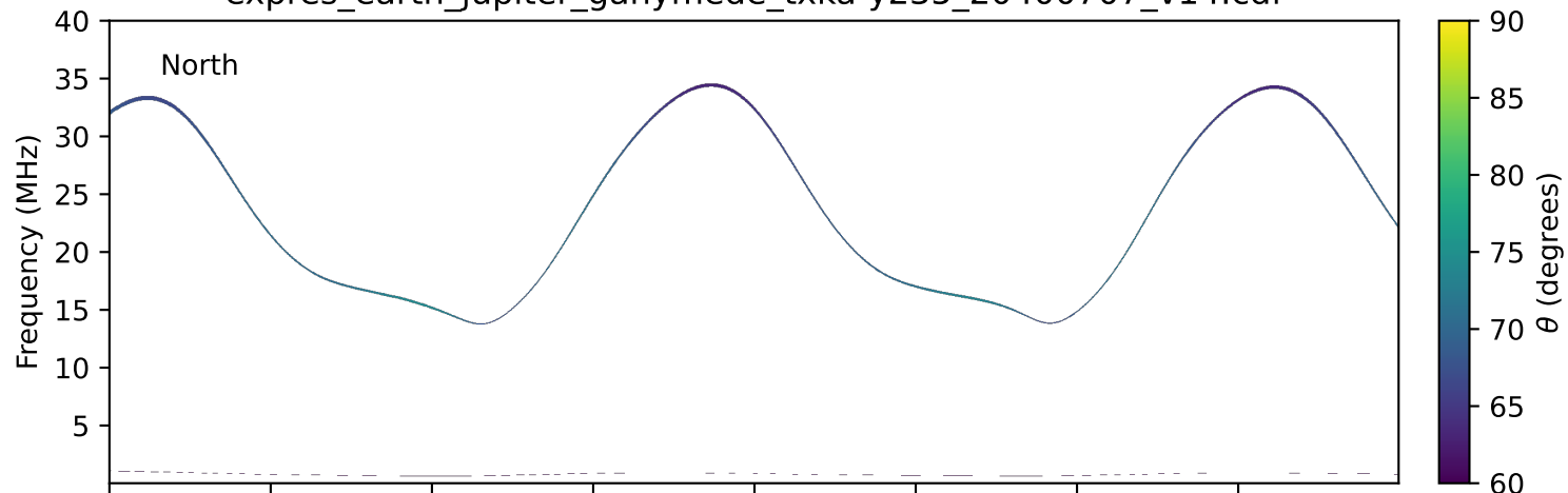
expres_earth_jupiter_ganymede_txka-y235_20400707_v14.cdf
