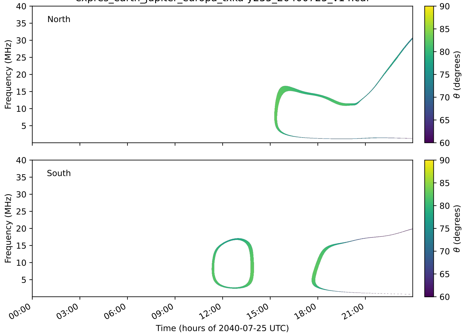
expres_earth_jupiter_europa_txka-y235_20400725_v14.cdf
