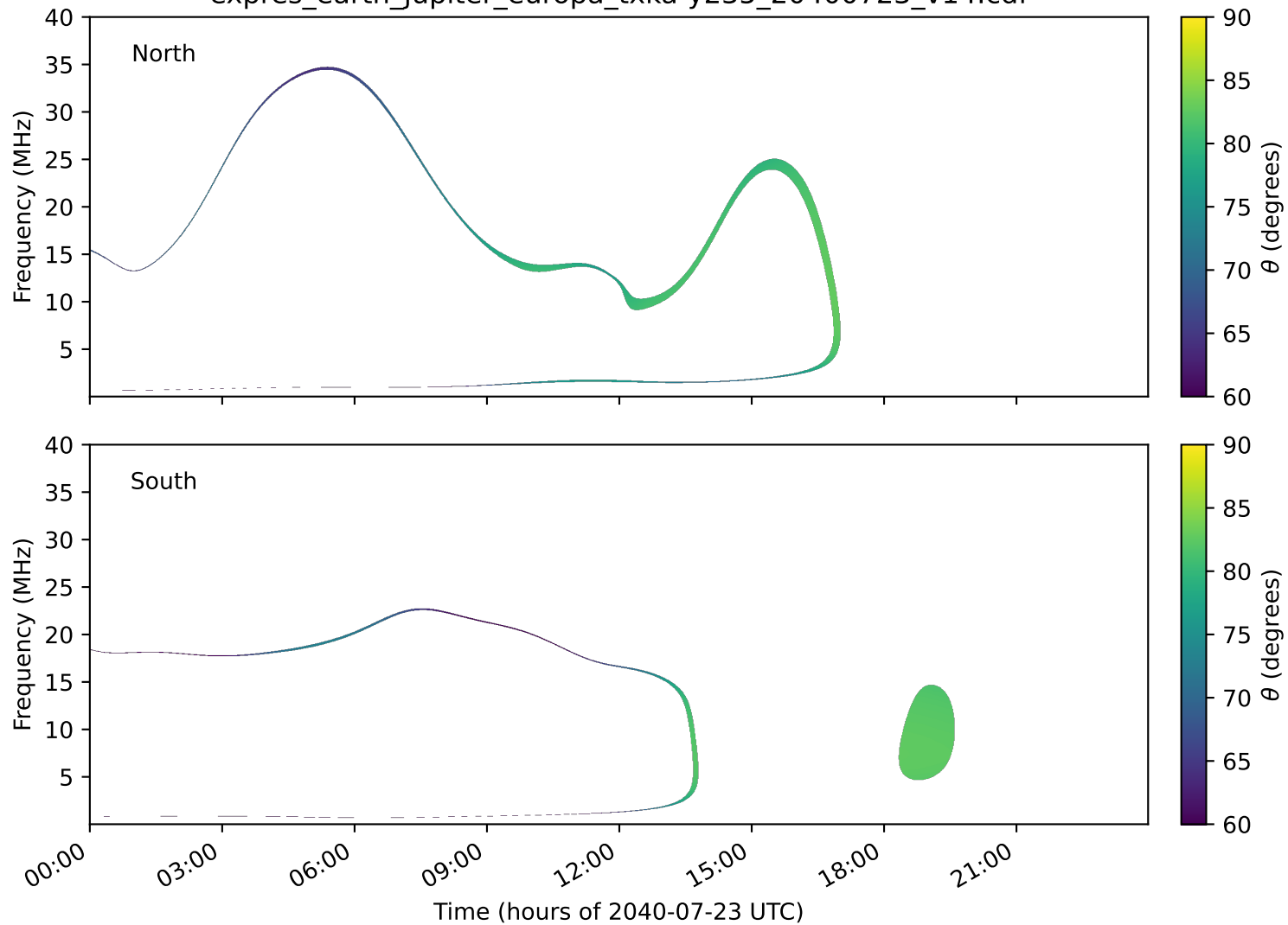
expres_earth_jupiter_europa_txka-y235_20400723_v14.cdf
