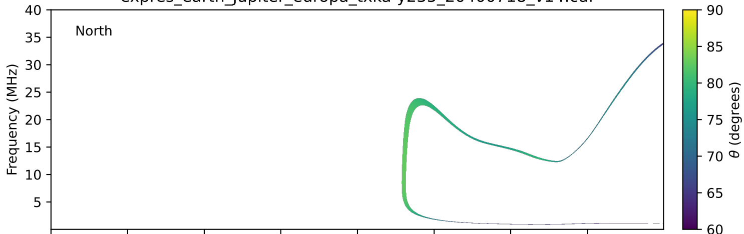
expres_earth_jupiter_europa_txka-y235_20400718_v14.cdf
