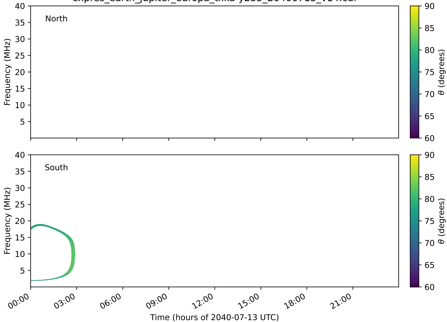
expres_earth_jupiter_europa_txka-y235_20400713_v14.cdf
