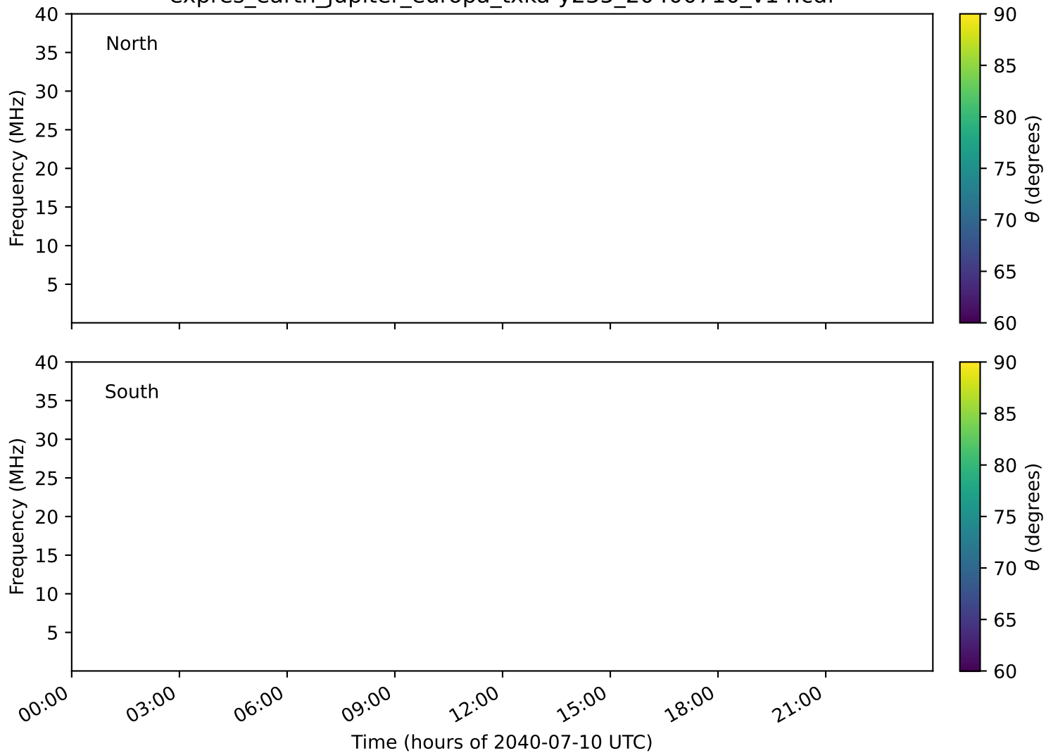
expres_earth_jupiter_europa_txka-y235_20400710_v14.cdf
