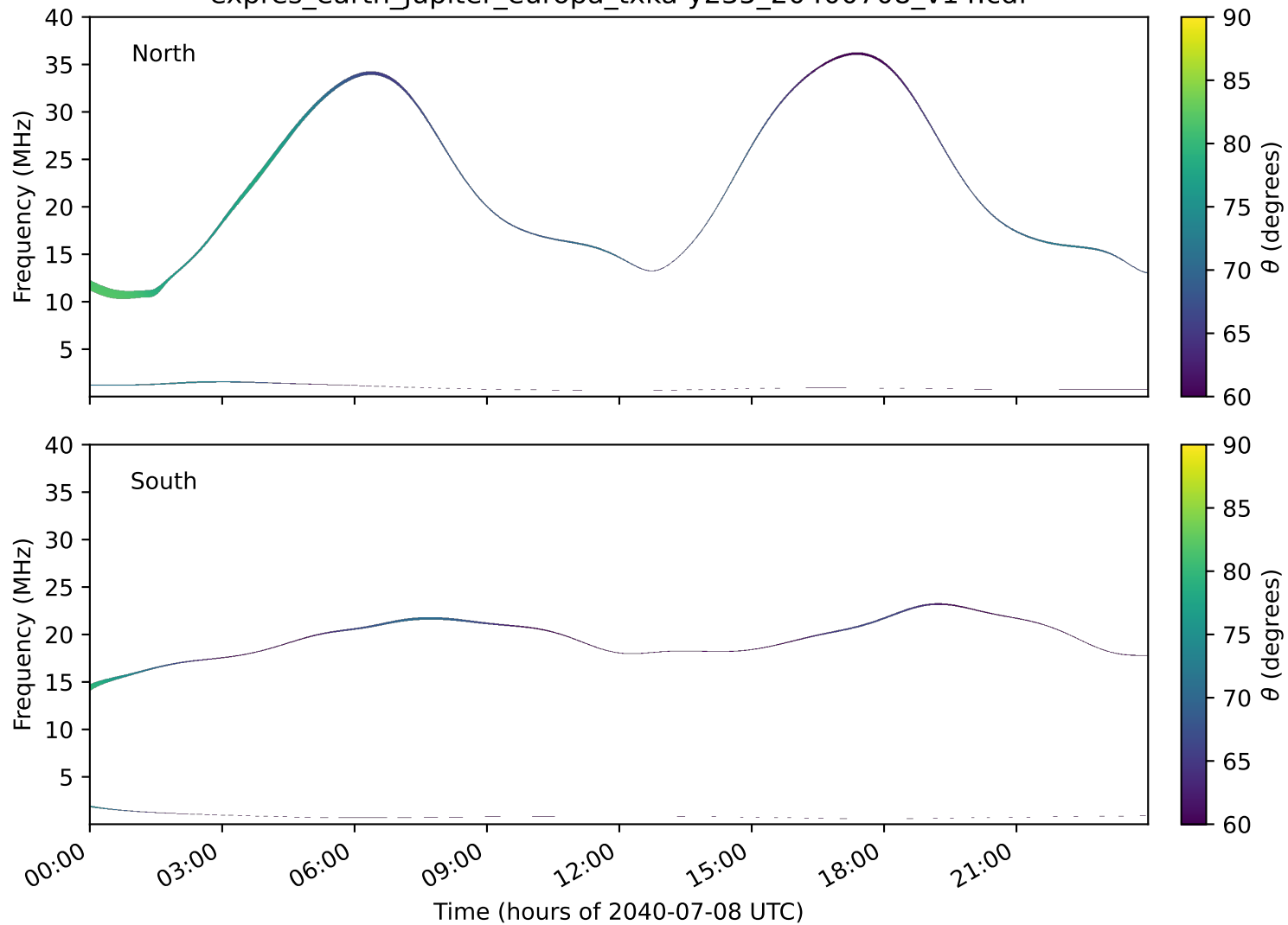
expres_earth_jupiter_europa_txka-y235_20400708_v14.cdf
