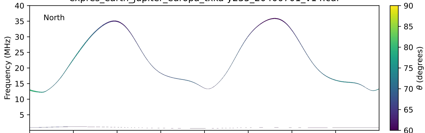
expres_earth_jupiter_europa_txka-y235_20400701_v14.cdf
