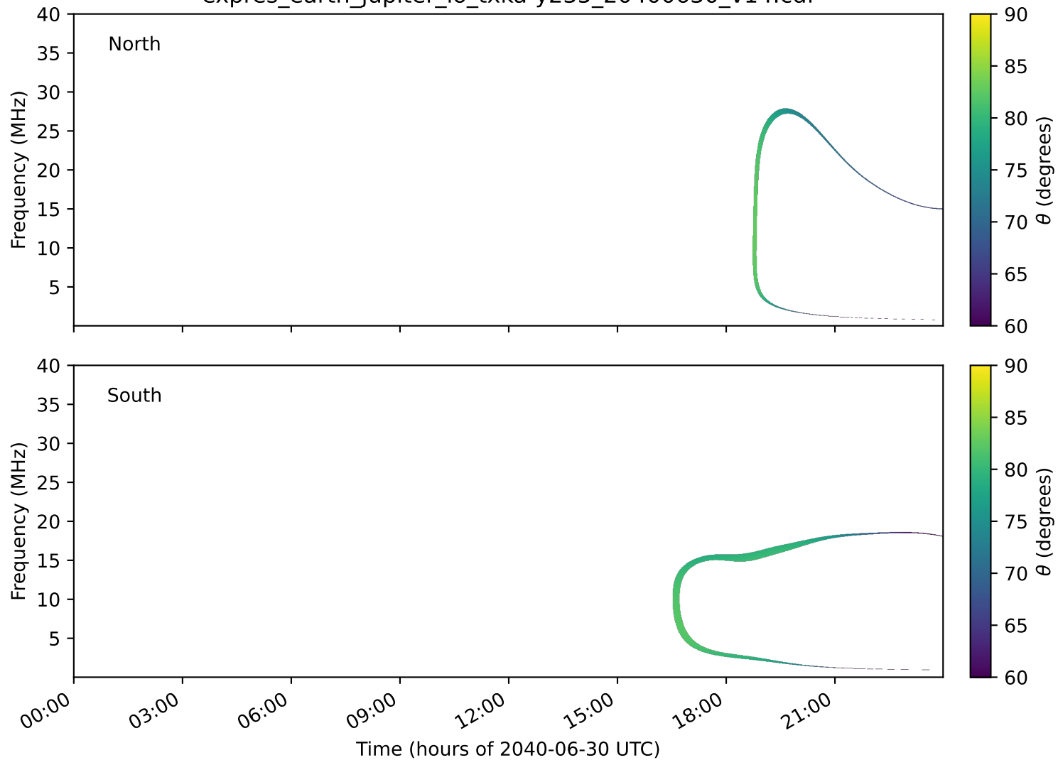
expres_earth_jupiter_io_txka-y235_20400630_v14.cdf
