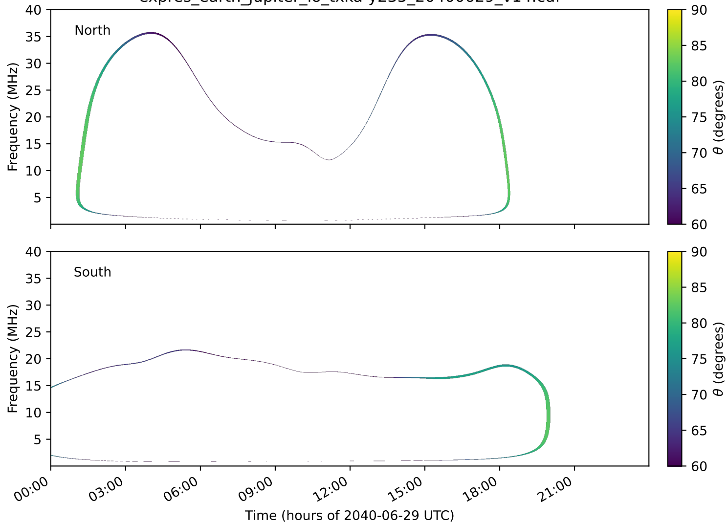
expres_earth_jupiter_io_txka-y235_20400629_v14.cdf
