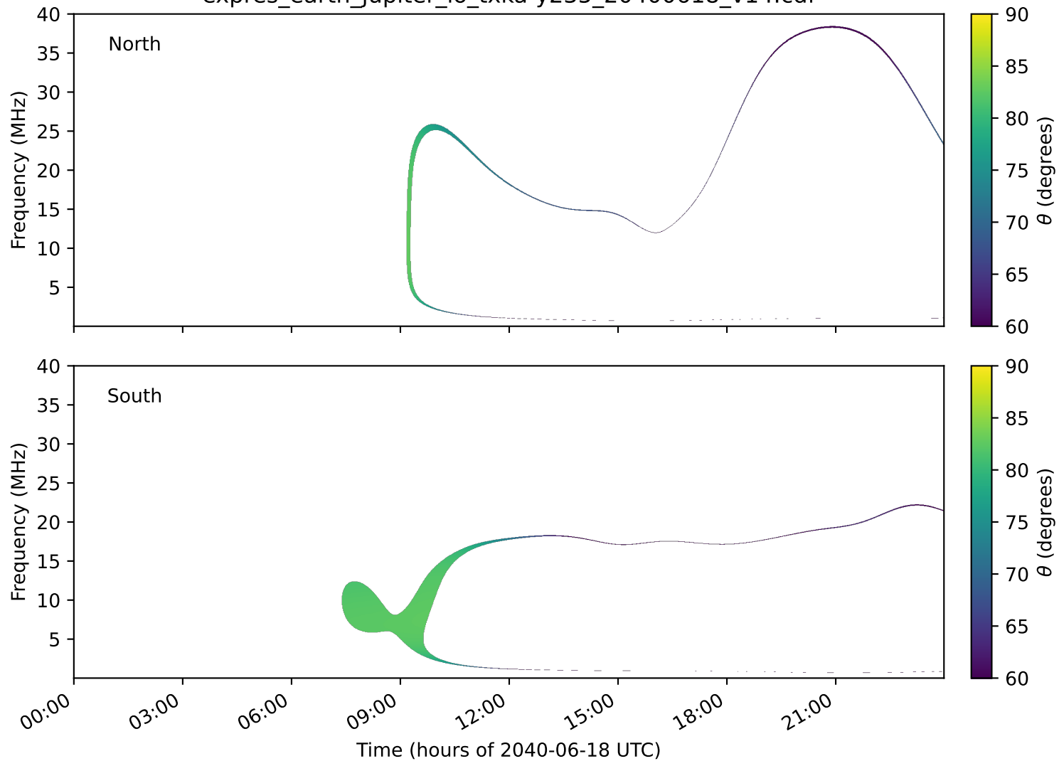
expres_earth_jupiter_io_txka-y235_20400618_v14.cdf
