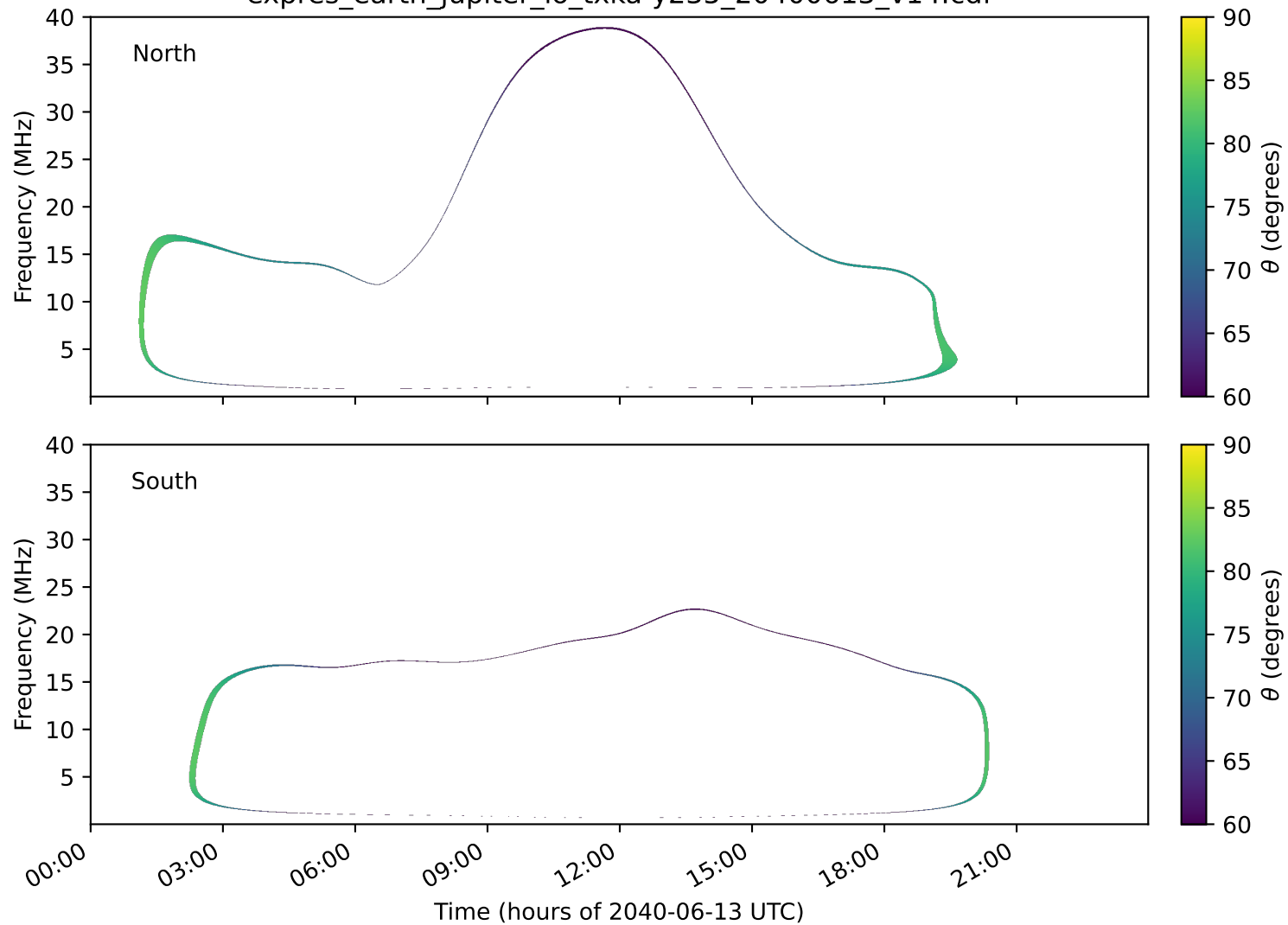
expres_earth_jupiter_io_txka-y235_20400613_v14.cdf
