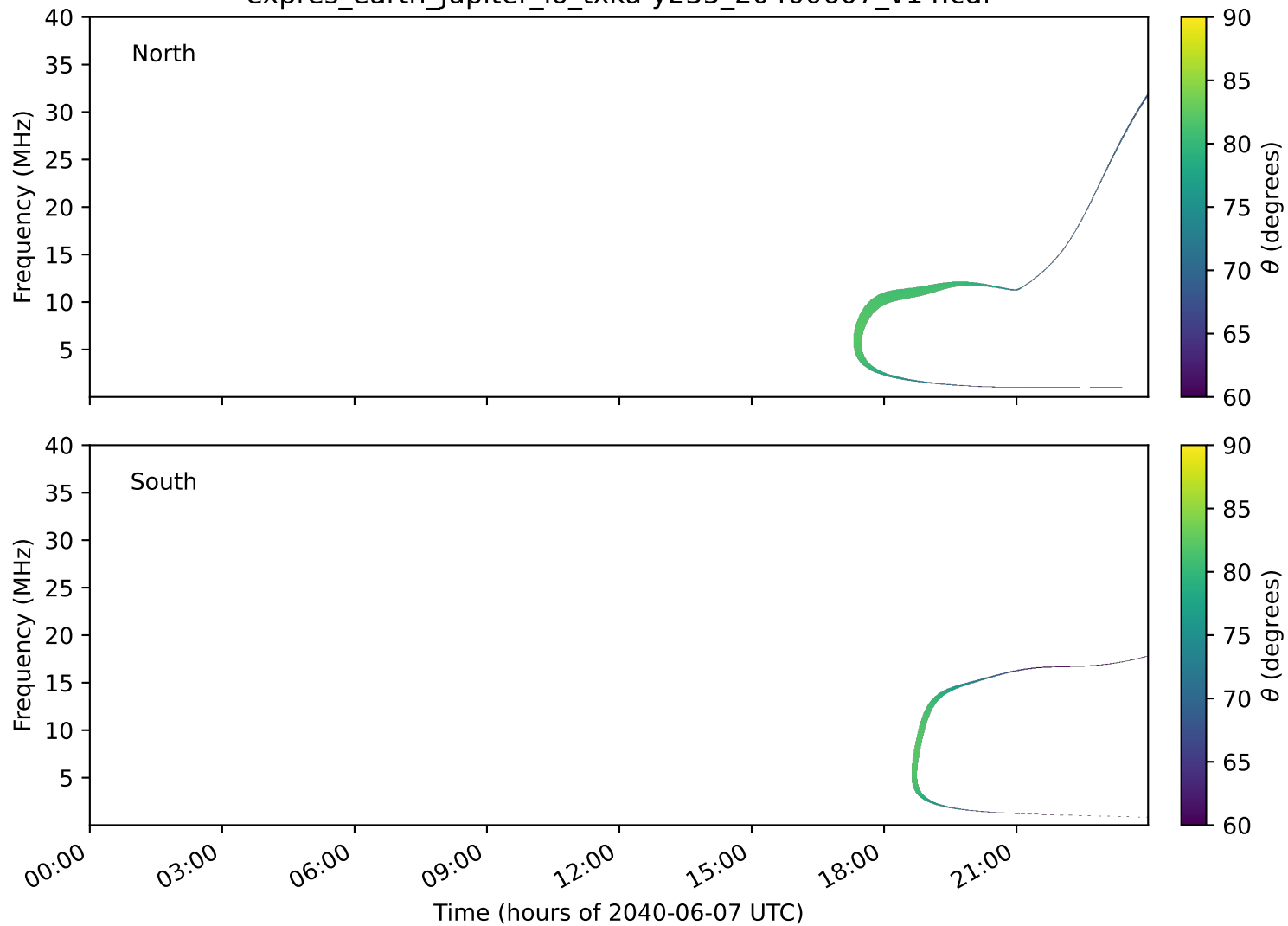
expres_earth_jupiter_io_txka-y235_20400607_v14.cdf
