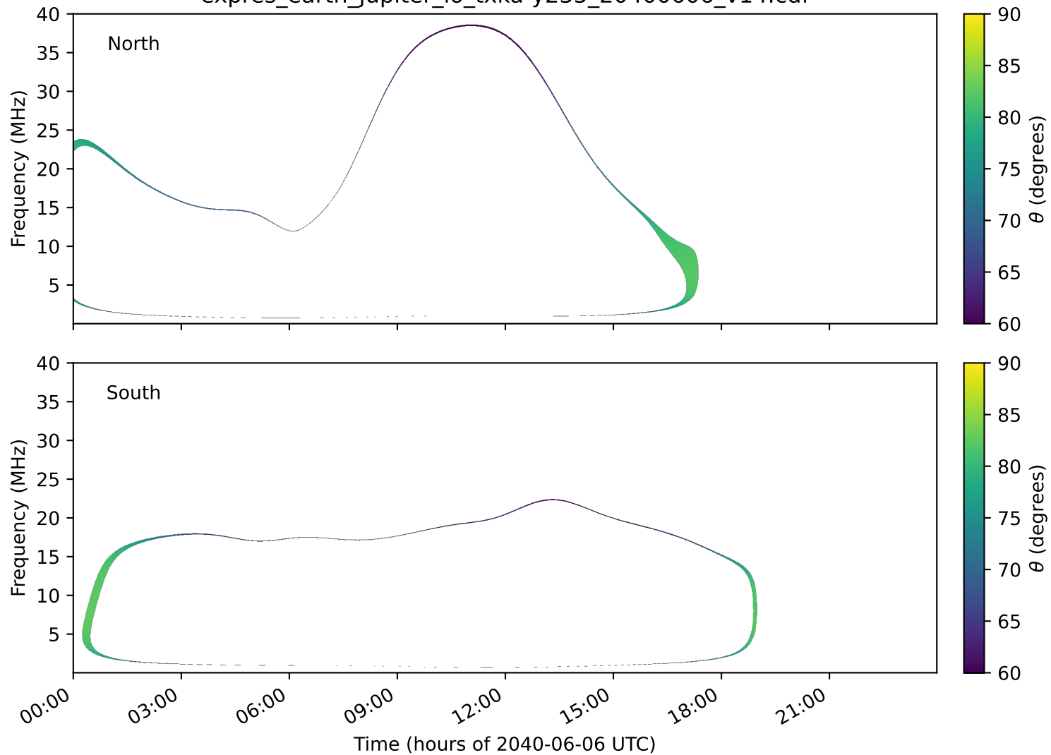
expres_earth_jupiter_io_txka-y235_20400606_v14.cdf
