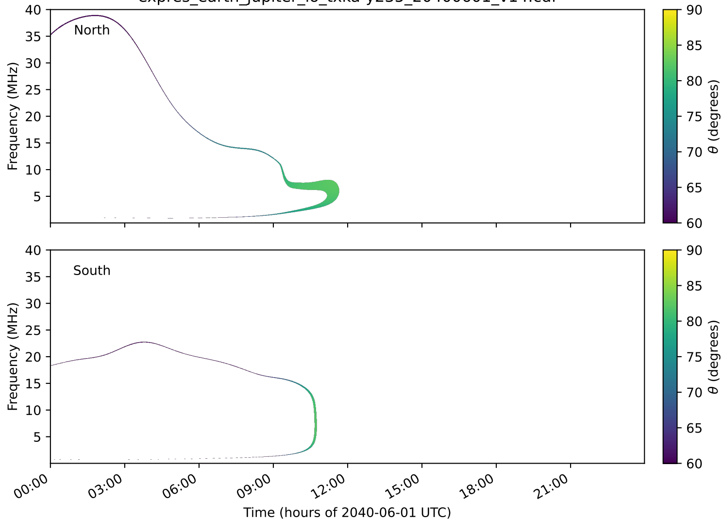
expres_earth_jupiter_io_txka-y235_20400601_v14.cdf
