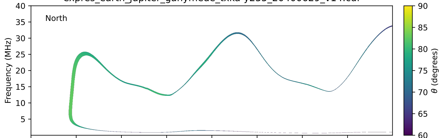
expres_earth_jupiter_ganymede_txka-y235_20400629_v14.cdf
