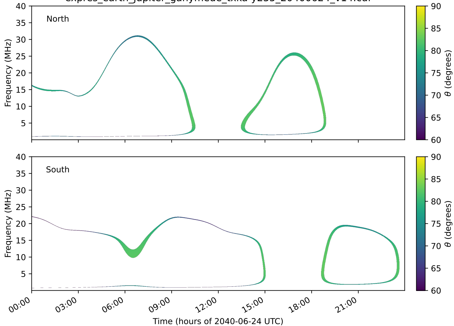
expres_earth_jupiter_ganymede_txka-y235_20400624_v14.cdf
