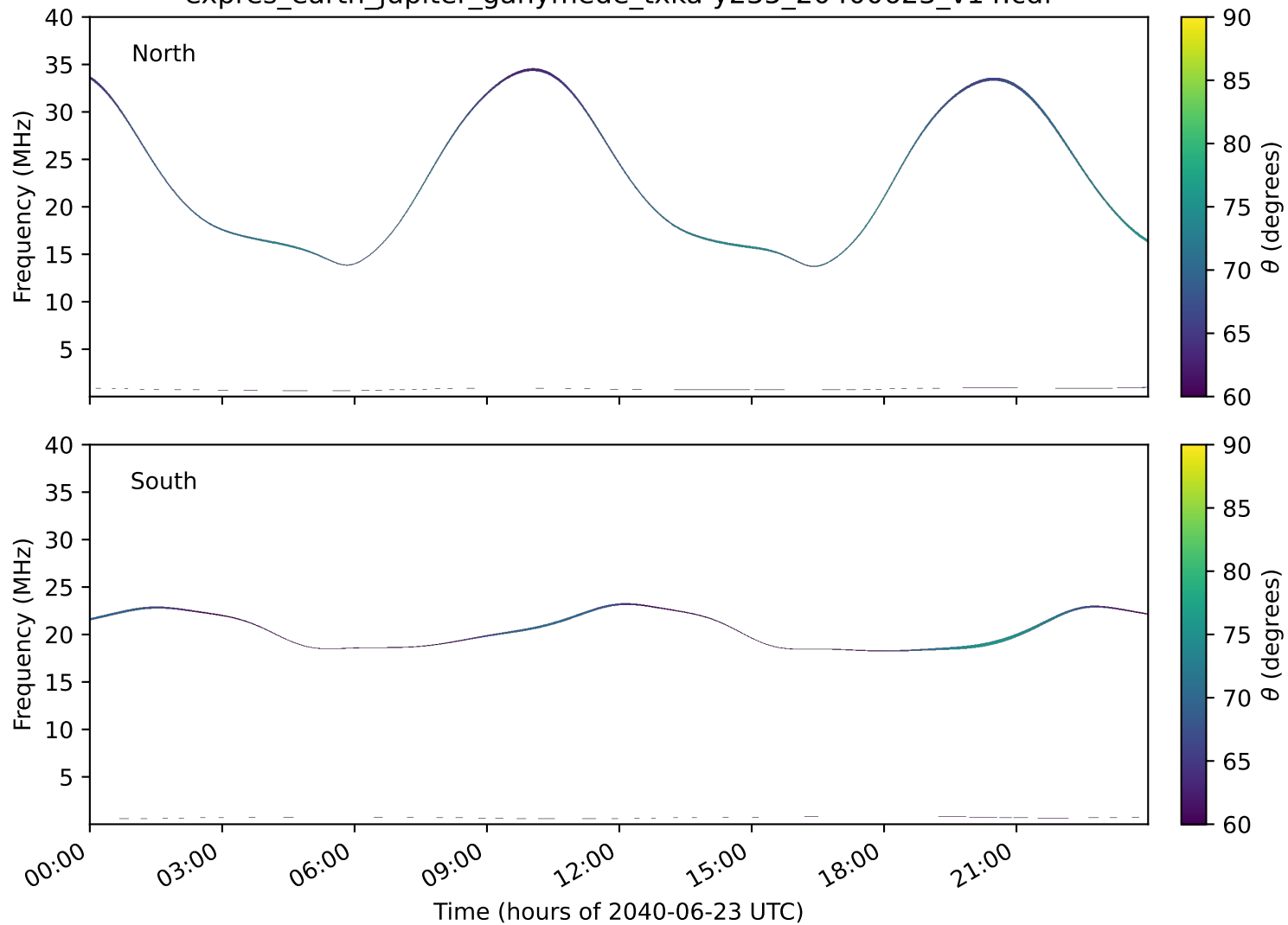
expres_earth_jupiter_ganymede_txka-y235_20400623_v14.cdf
