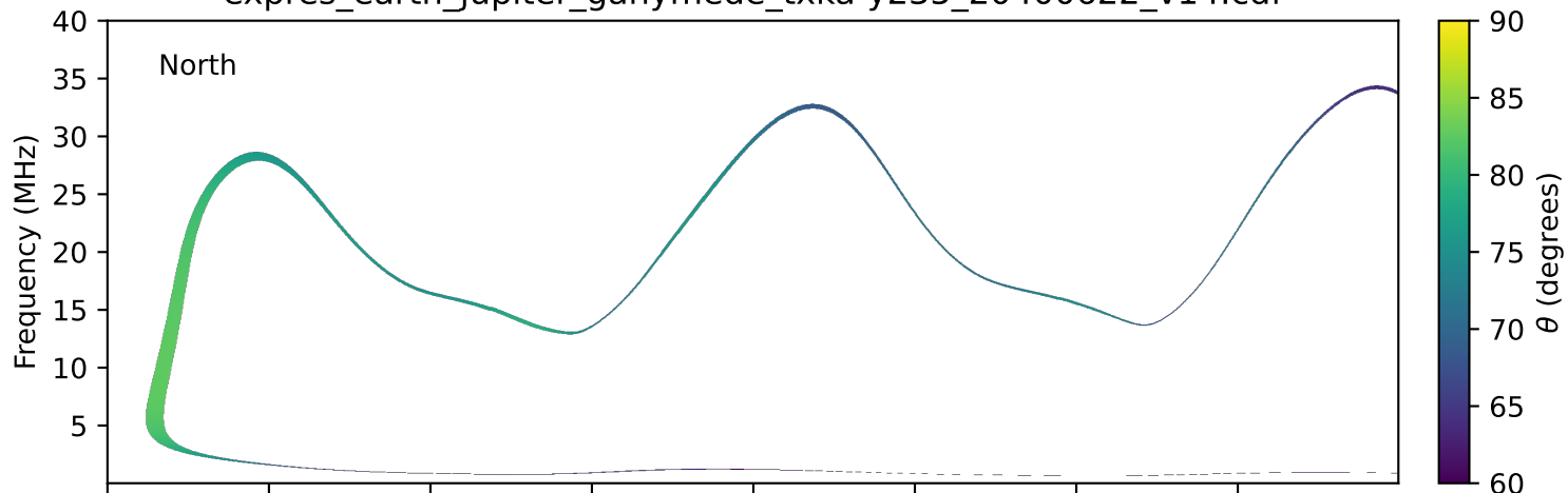
expres_earth_jupiter_ganymede_txka-y235_20400622_v14.cdf
