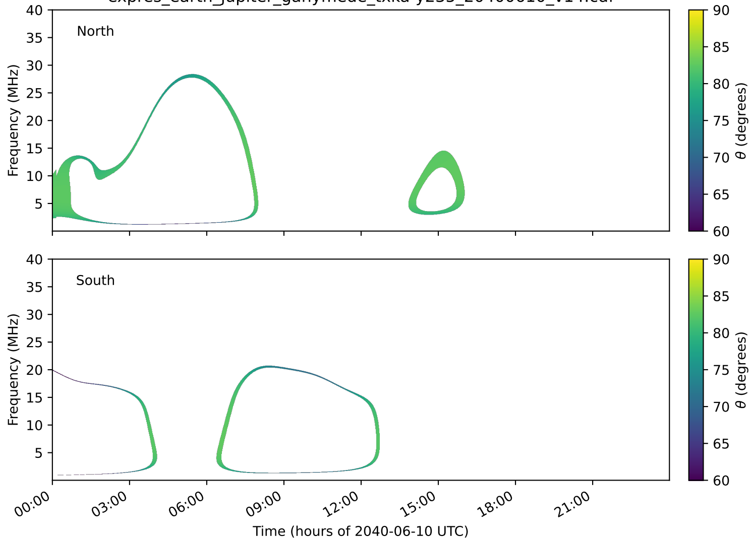
expres_earth_jupiter_ganymede_txka-y235_20400610_v14.cdf
