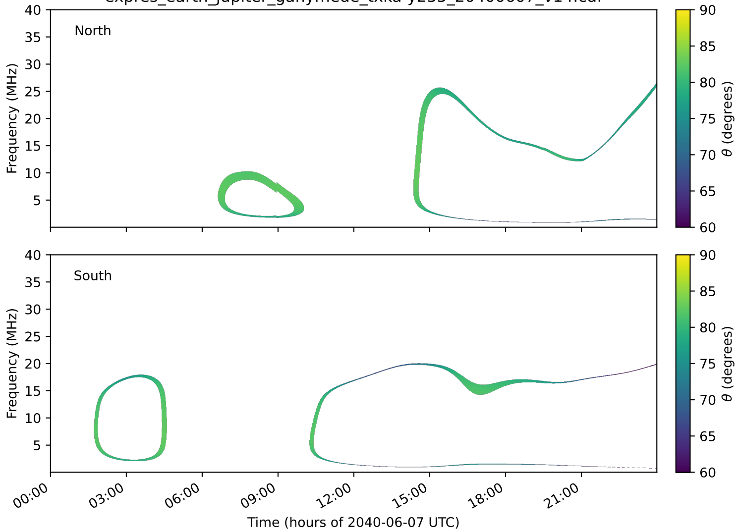
expres_earth_jupiter_ganymede_txka-y235_20400607_v14.cdf
