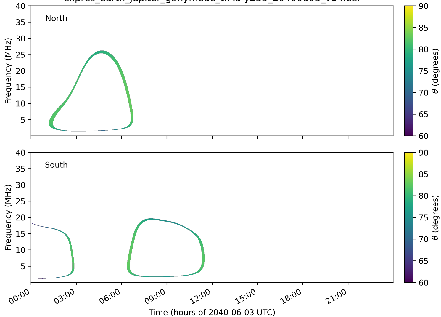
expres_earth_jupiter_ganymede_txka-y235_20400603_v14.cdf
