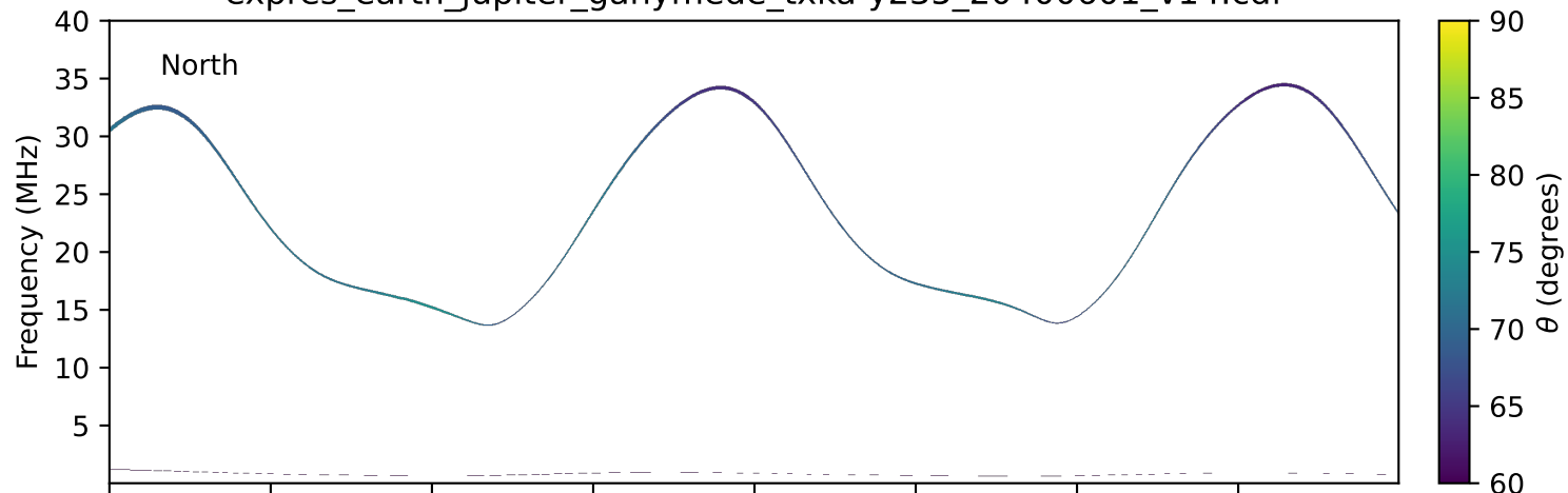
expres_earth_jupiter_ganymede_txka-y235_20400601_v14.cdf
