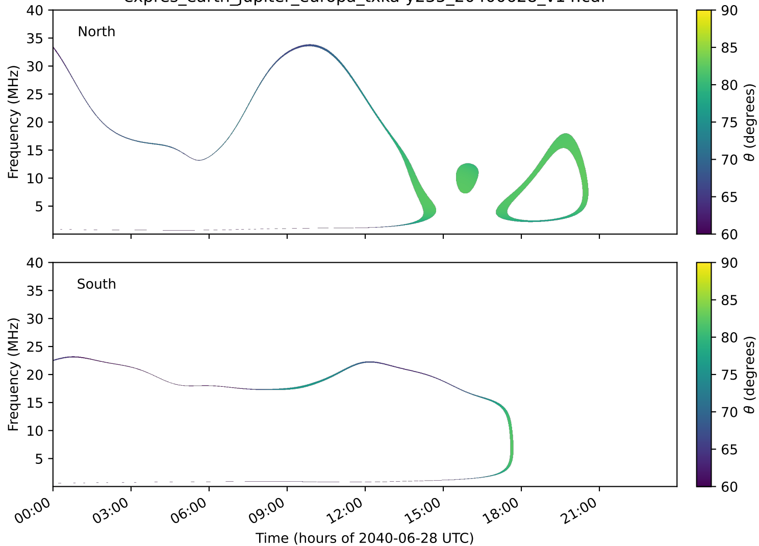
expres_earth_jupiter_europa_txka-y235_20400628_v14.cdf
