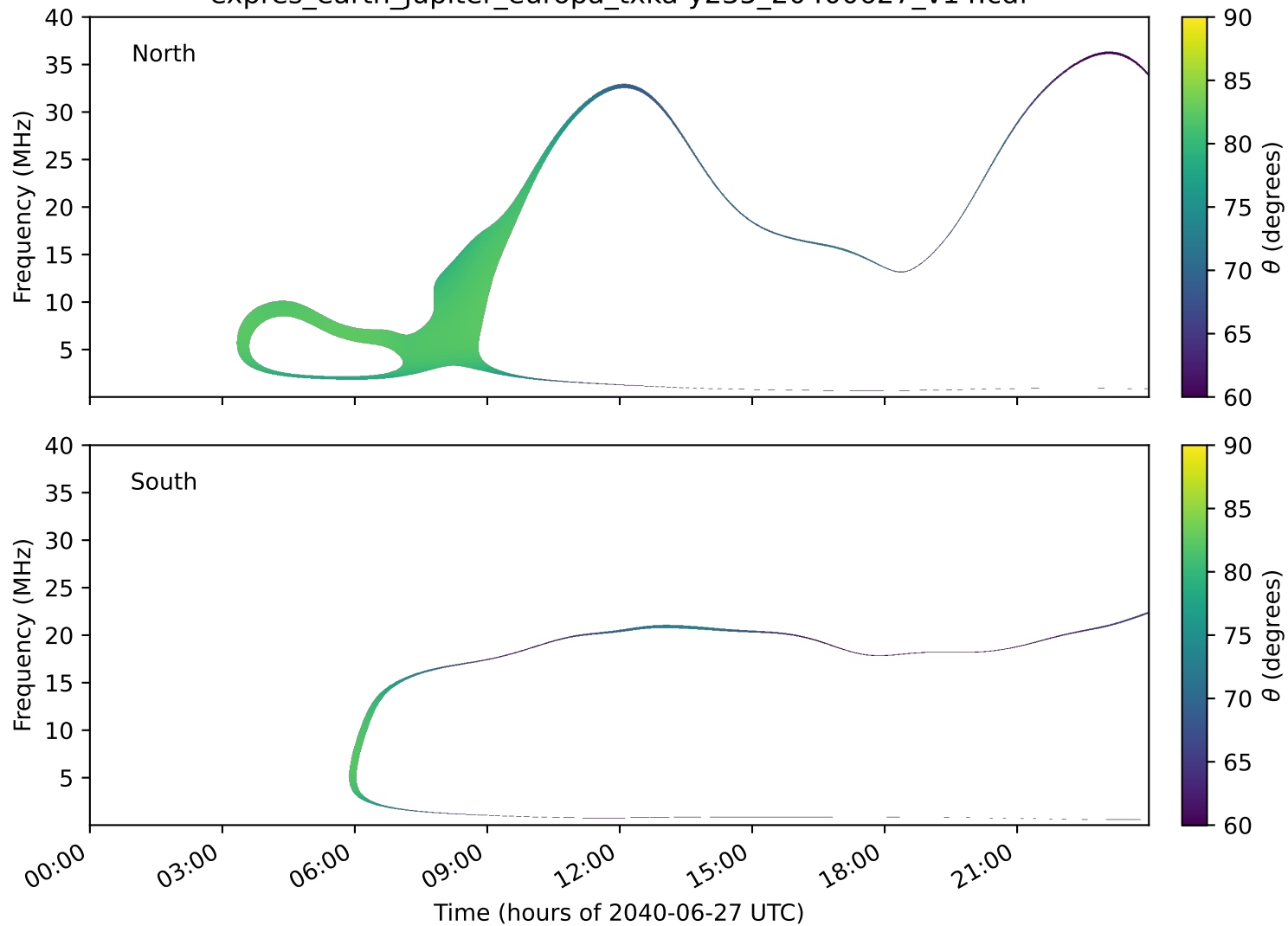
expres_earth_jupiter_europa_txka-y235_20400627_v14.cdf
