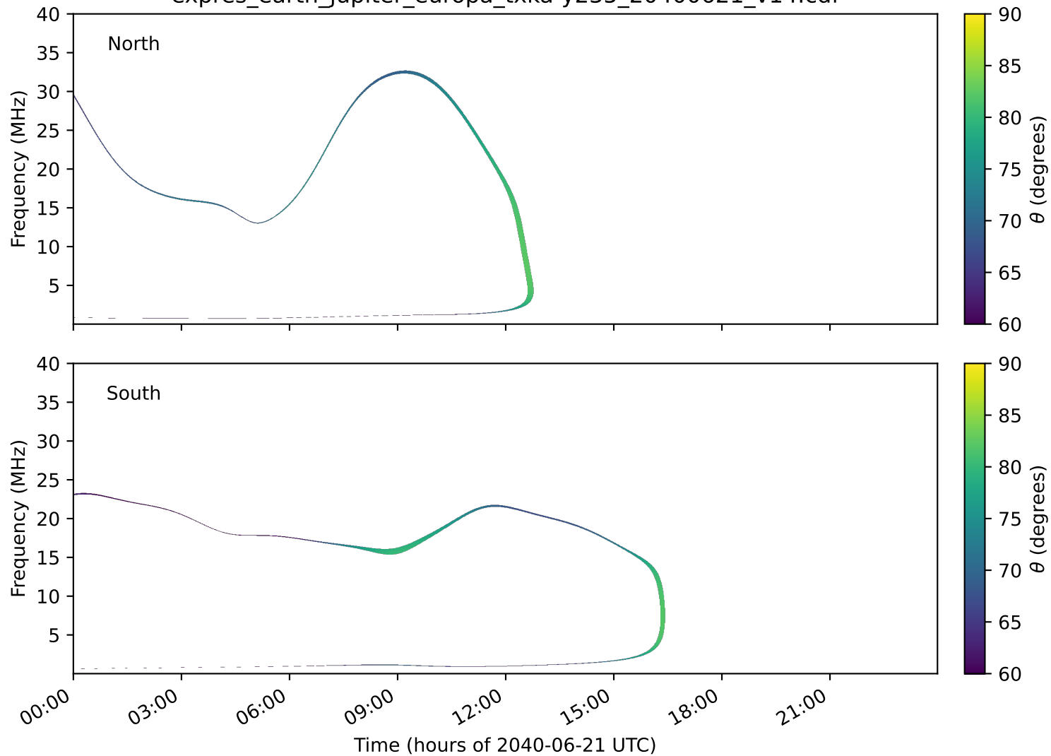
expres_earth_jupiter_europa_txka-y235_20400621_v14.cdf
