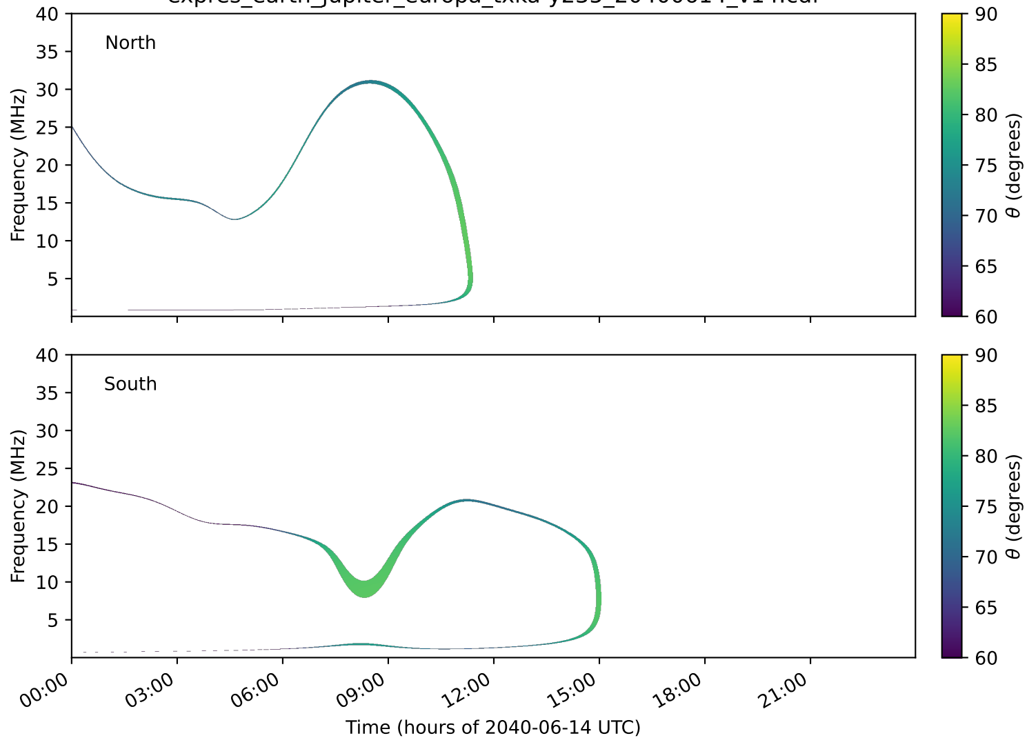
expres_earth_jupiter_europa_txka-y235_20400614_v14.cdf
