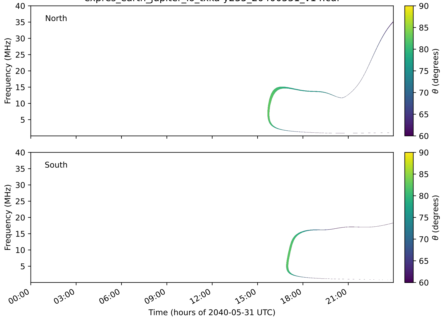
expres_earth_jupiter_io_txka-y235_20400531_v14.cdf
