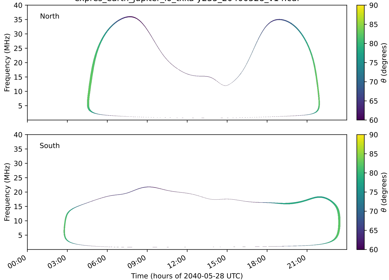
expres_earth_jupiter_io_txka-y235_20400528_v14.cdf
