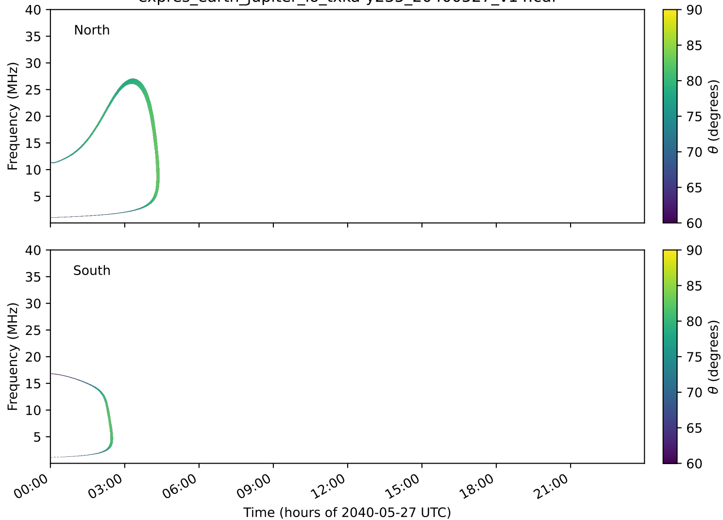
expres_earth_jupiter_io_txka-y235_20400527_v14.cdf
