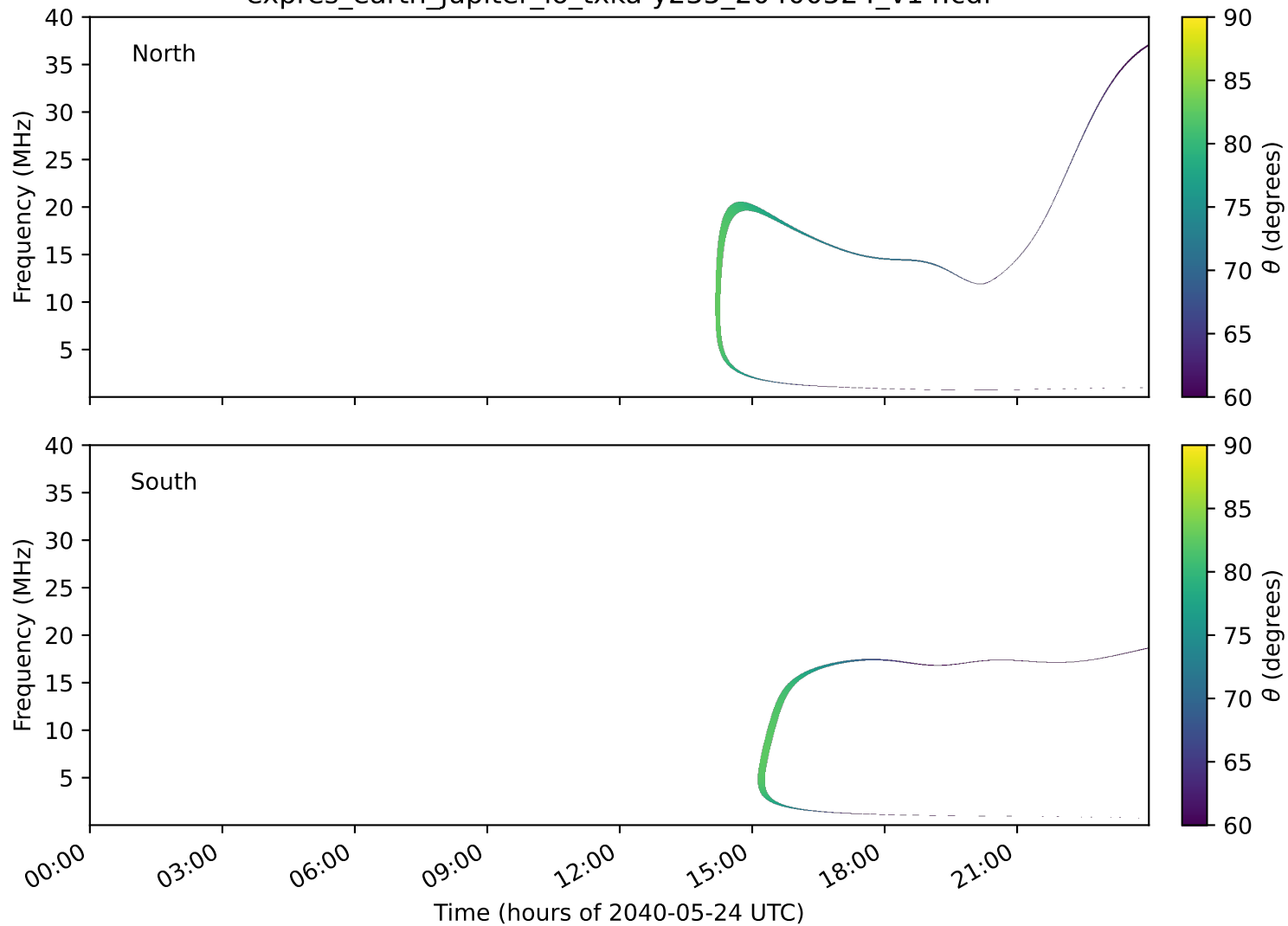
expres_earth_jupiter_io_txka-y235_20400524_v14.cdf
