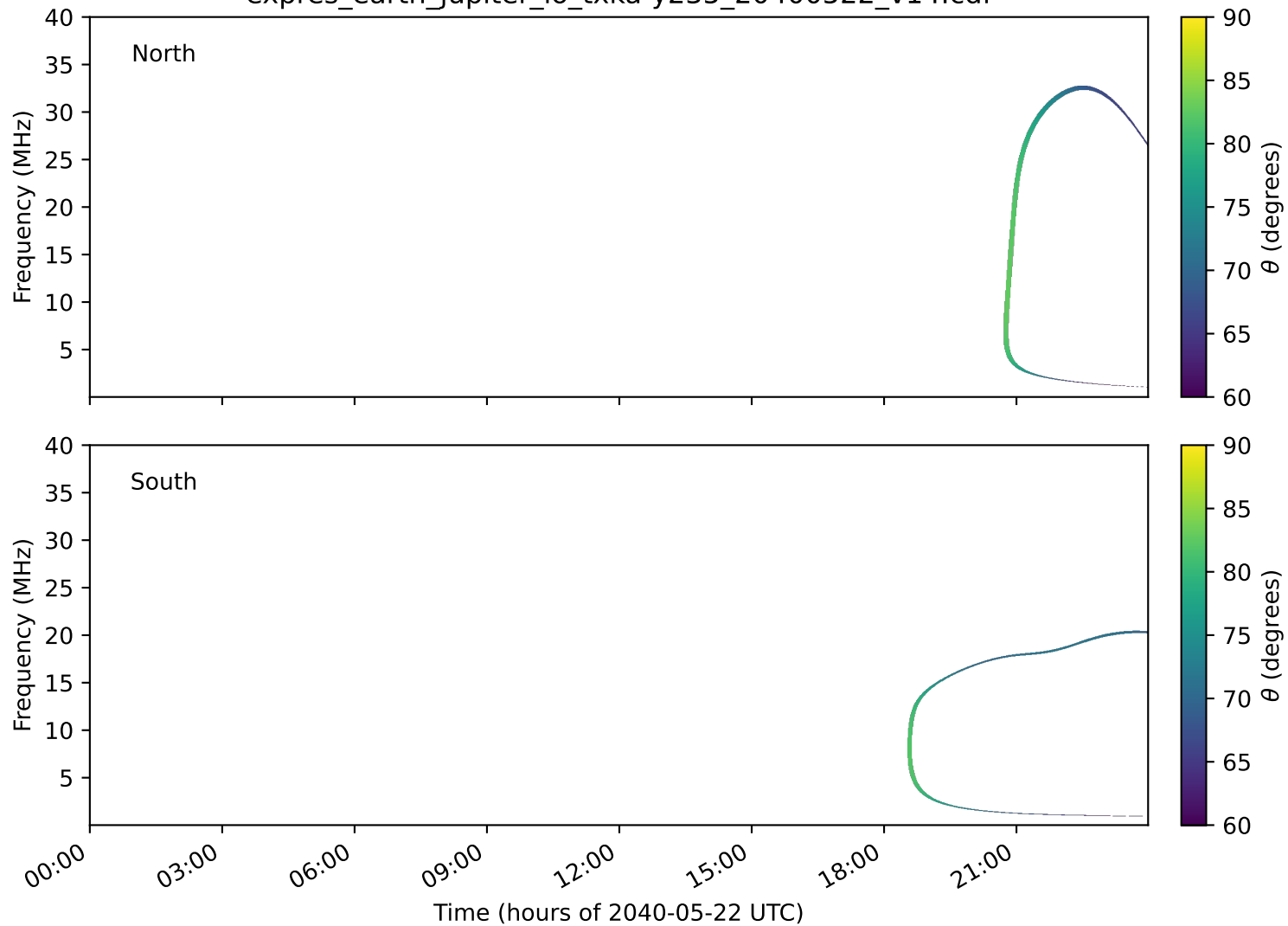
expres_earth_jupiter_io_txka-y235_20400522_v14.cdf
