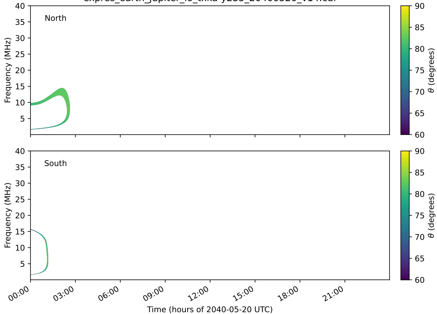
expres_earth_jupiter_io_txka-y235_20400520_v14.cdf
