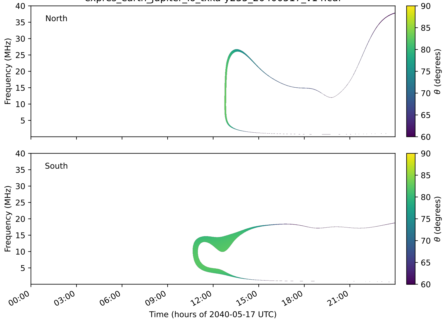
expres_earth_jupiter_io_txka-y235_20400517_v14.cdf
