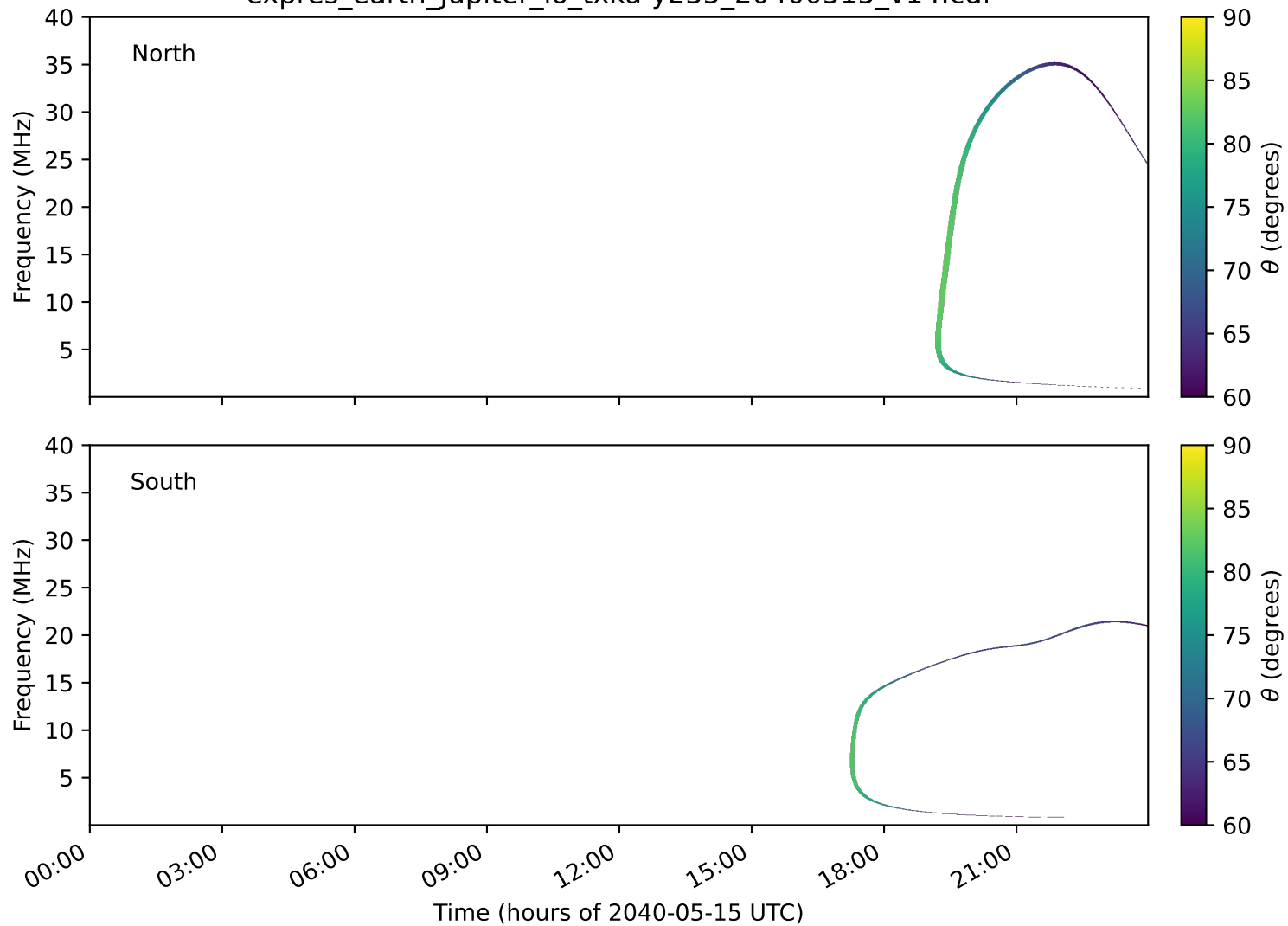
expres_earth_jupiter_io_txka-y235_20400515_v14.cdf
