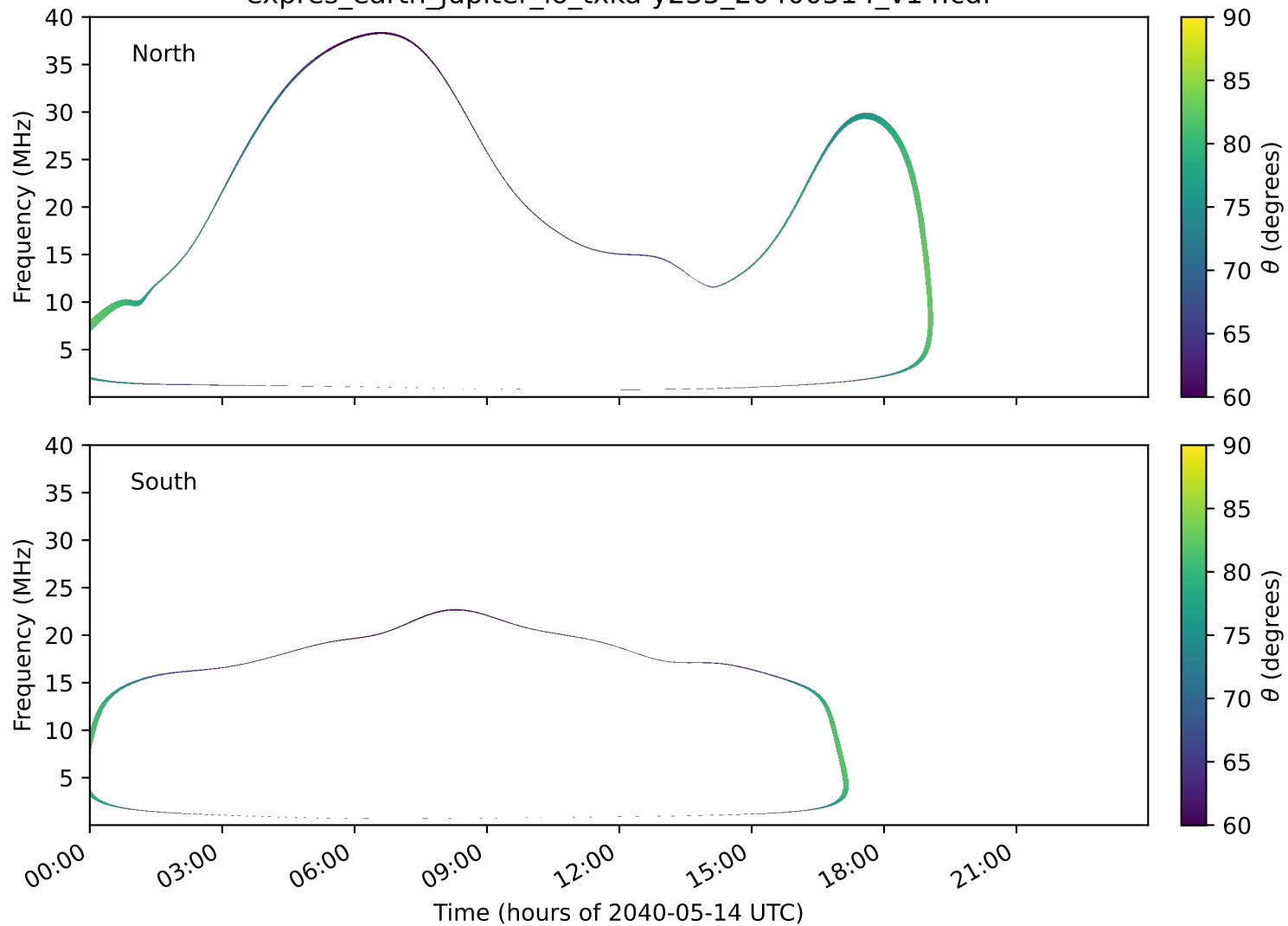
expres_earth_jupiter_io_txka-y235_20400514_v14.cdf
