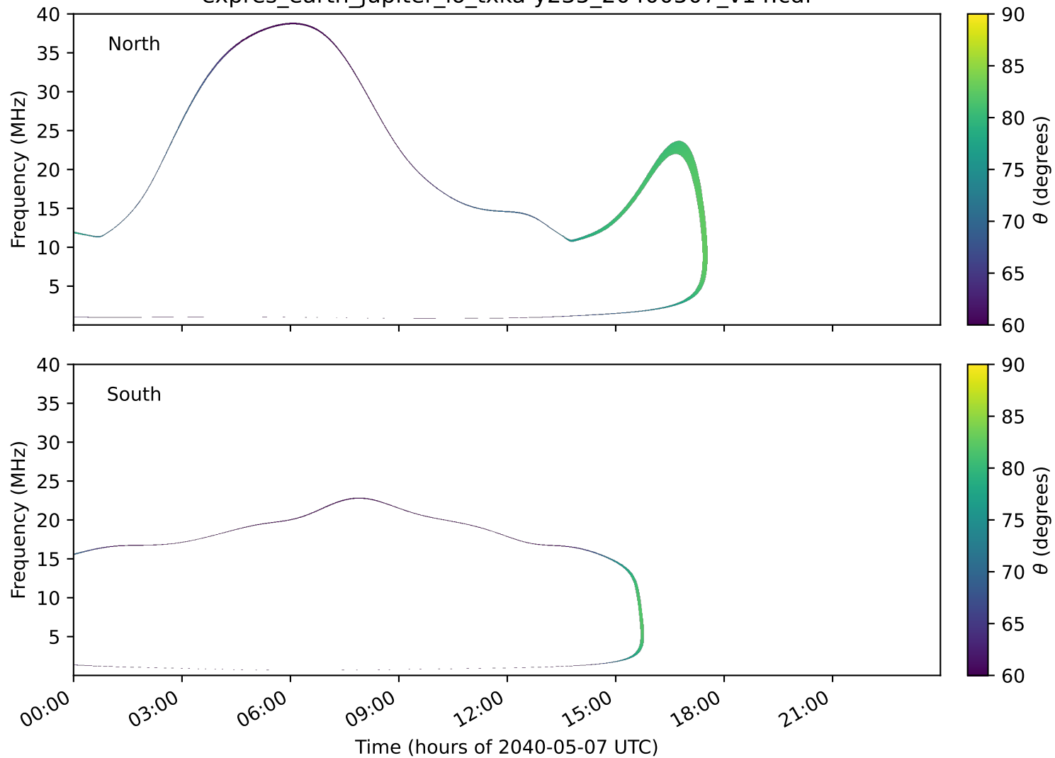
expres_earth_jupiter_io_txka-y235_20400507_v14.cdf
