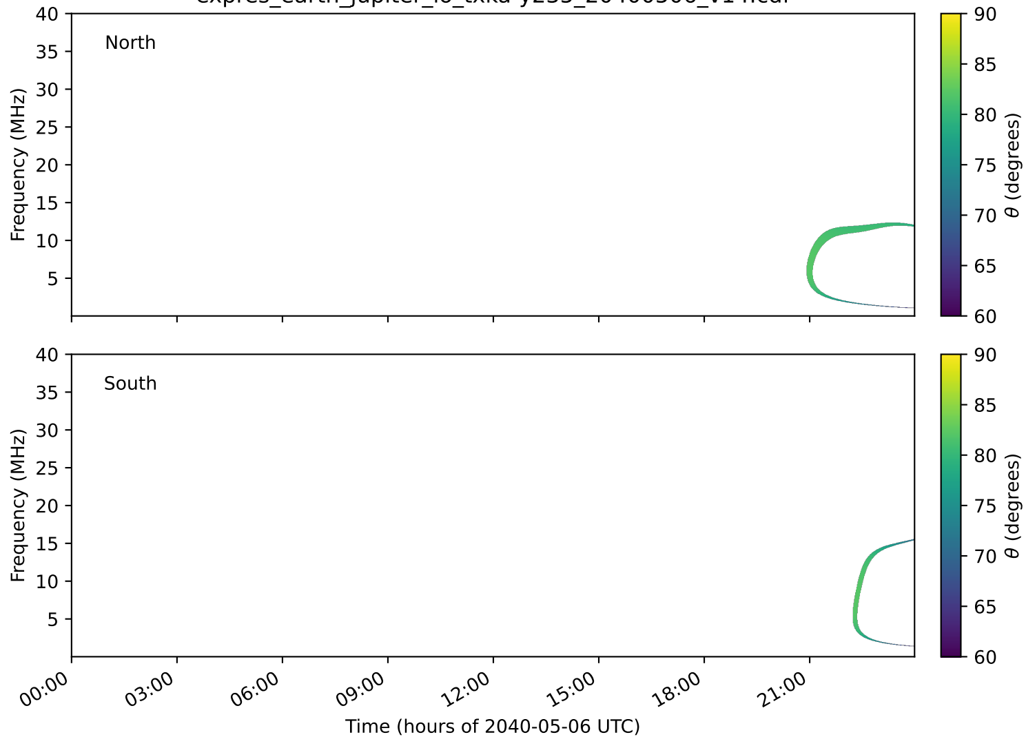
expres_earth_jupiter_io_txka-y235_20400506_v14.cdf
