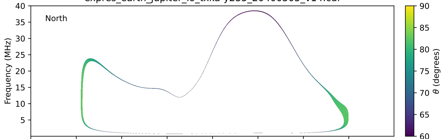
expres_earth_jupiter_io_txka-y235_20400505_v14.cdf
