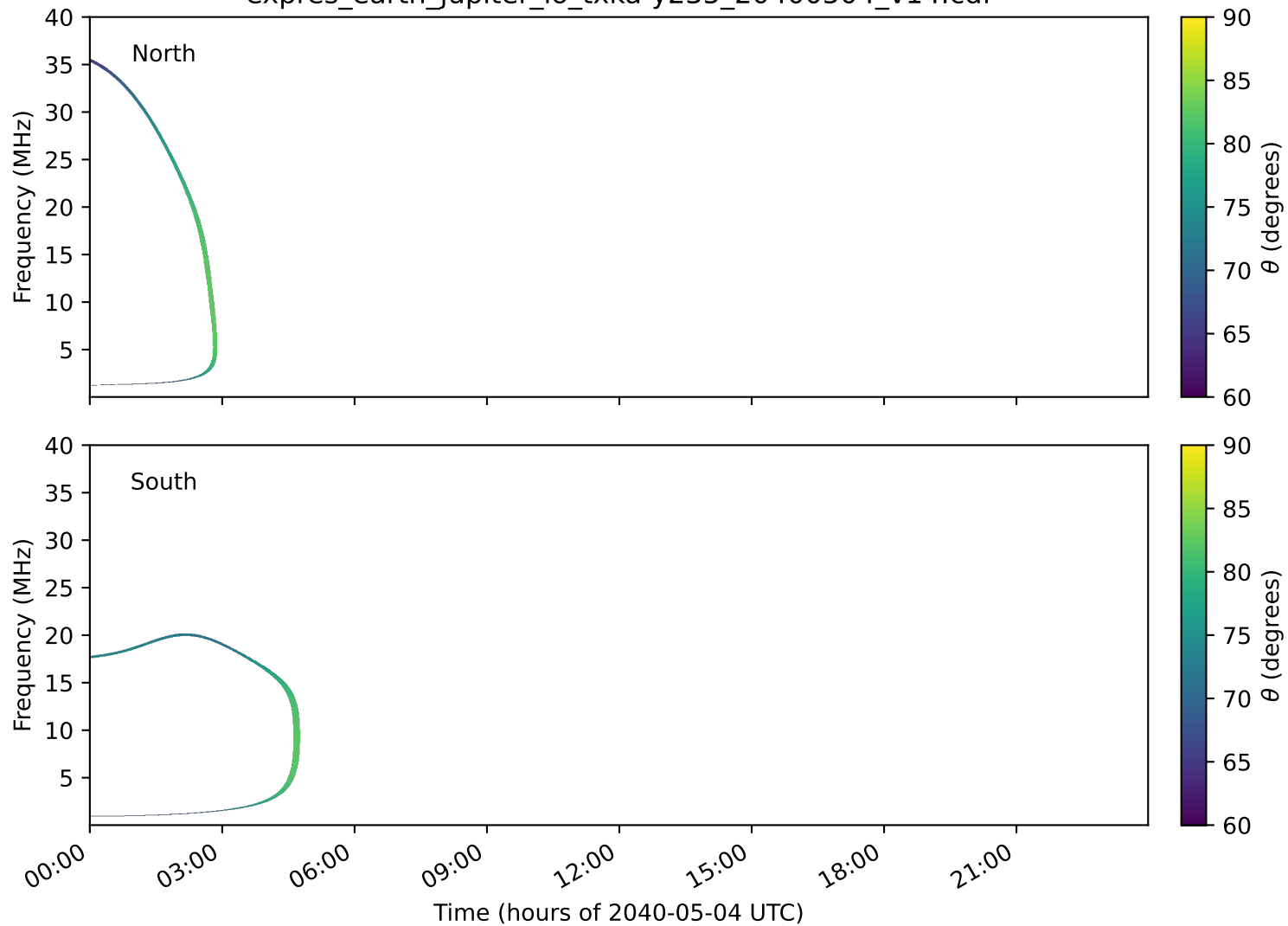
expres_earth_jupiter_io_txka-y235_20400504_v14.cdf
