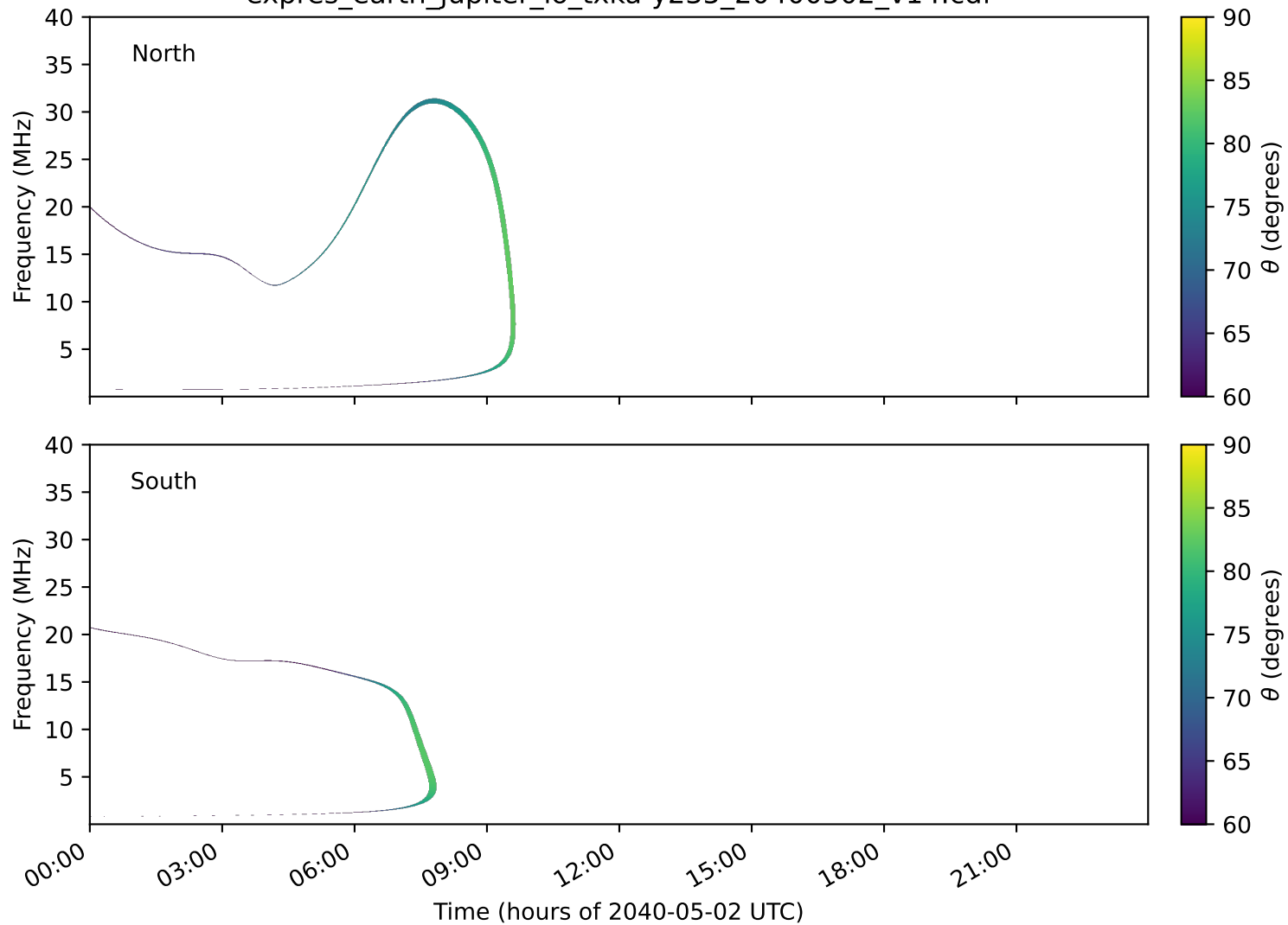
expres_earth_jupiter_io_txka-y235_20400502_v14.cdf
