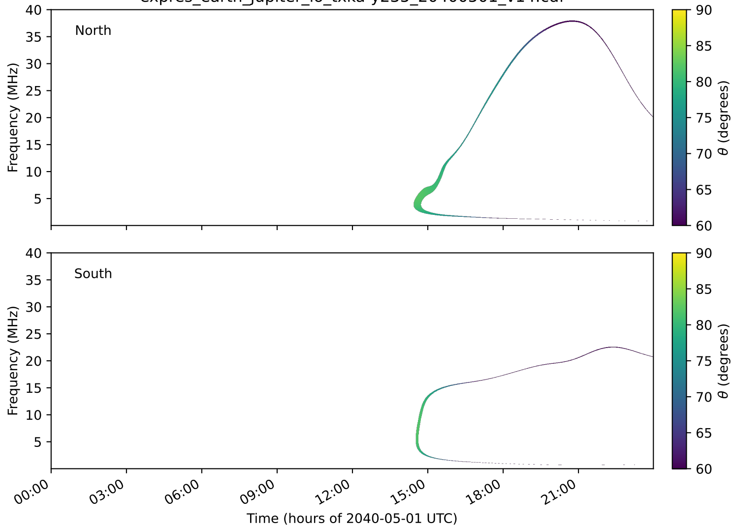
expres_earth_jupiter_io_txka-y235_20400501_v14.cdf
