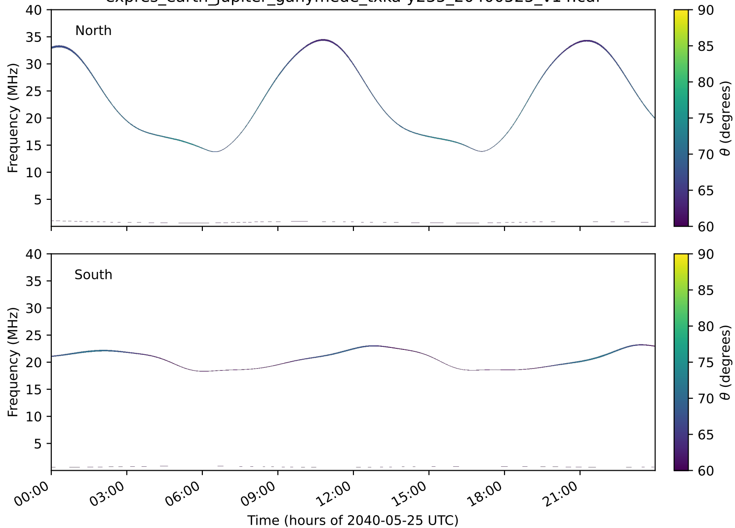
expres_earth_jupiter_ganymede_txka-y235_20400525_v14.cdf
