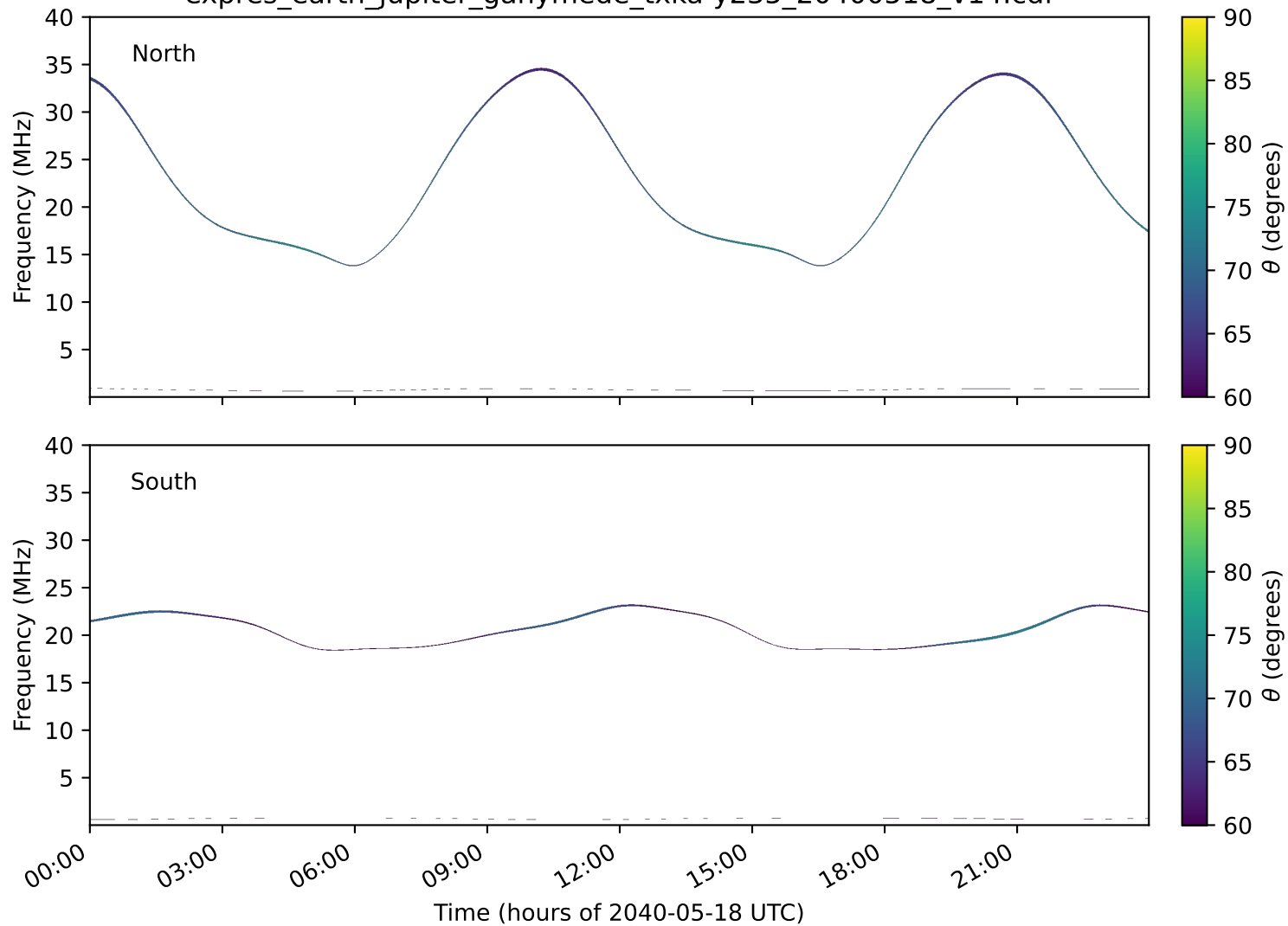
expres_earth_jupiter_ganymede_txka-y235_20400518_v14.cdf
