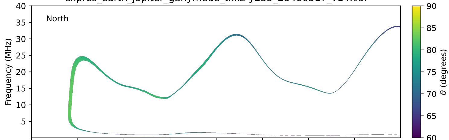
expres_earth_jupiter_ganymede_txka-y235_20400517_v14.cdf
