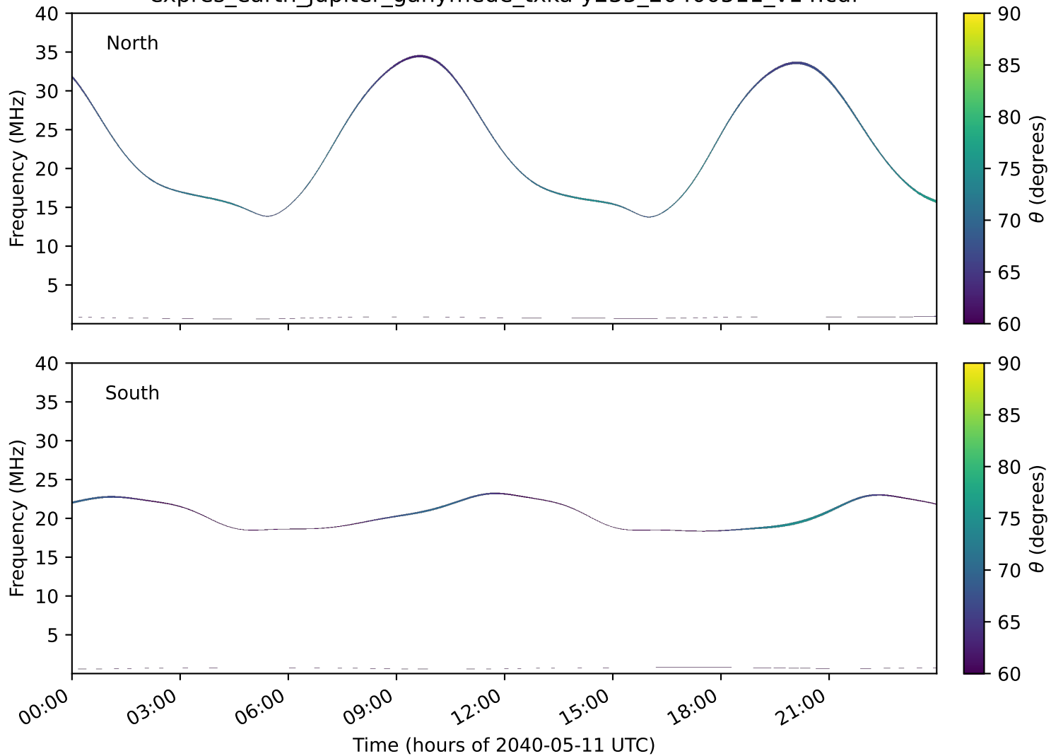
expres_earth_jupiter_ganymede_txka-y235_20400511_v14.cdf
