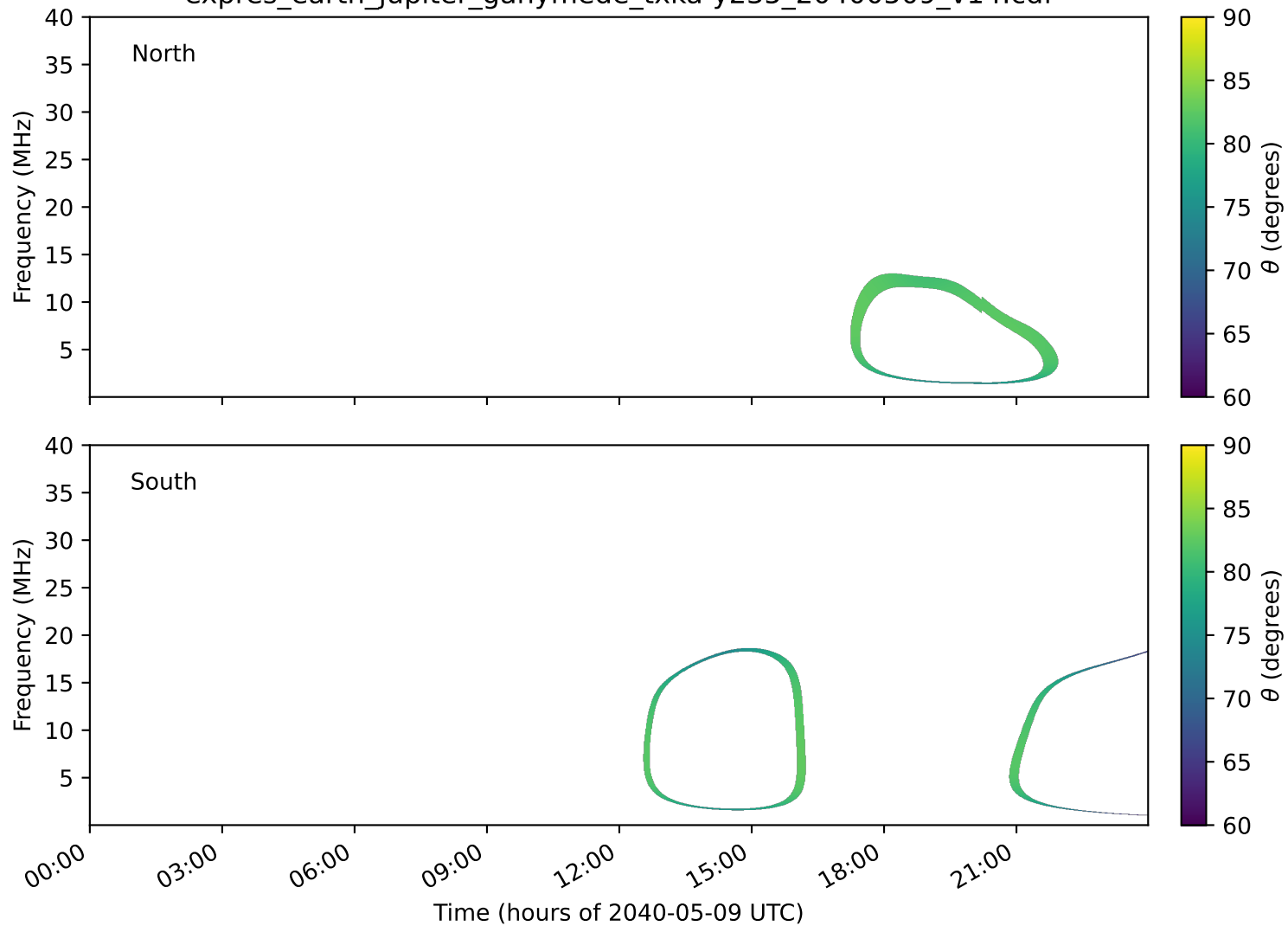
expres_earth_jupiter_ganymede_txka-y235_20400509_v14.cdf
