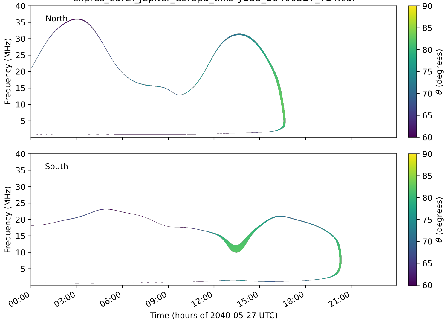
expres_earth_jupiter_europa_txka-y235_20400527_v14.cdf
